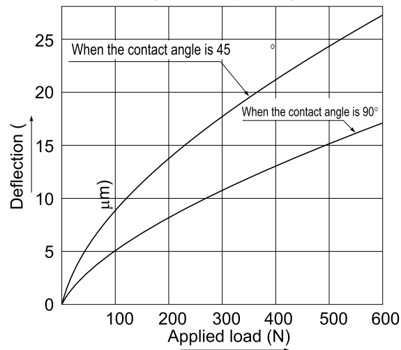
Fig.4 Radial Load and Deffection
