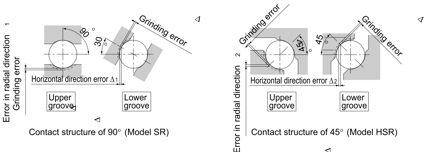
Fig.2 Machining Error and Accuracy
