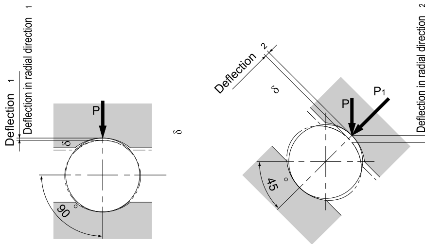
Fig.3 Deffection under a Radial Load
