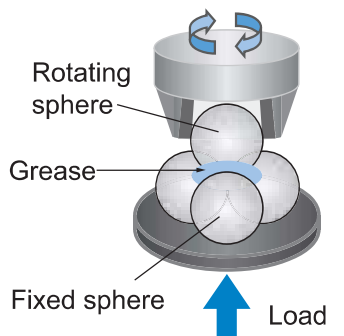
Testing apparatus
