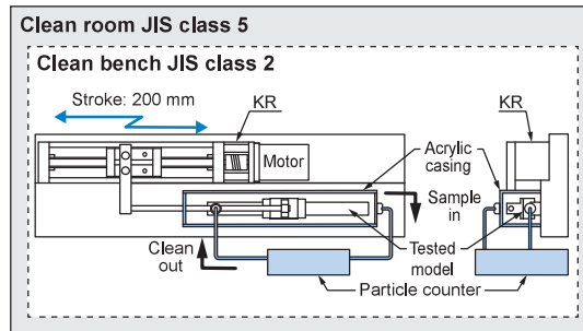
Testing device
