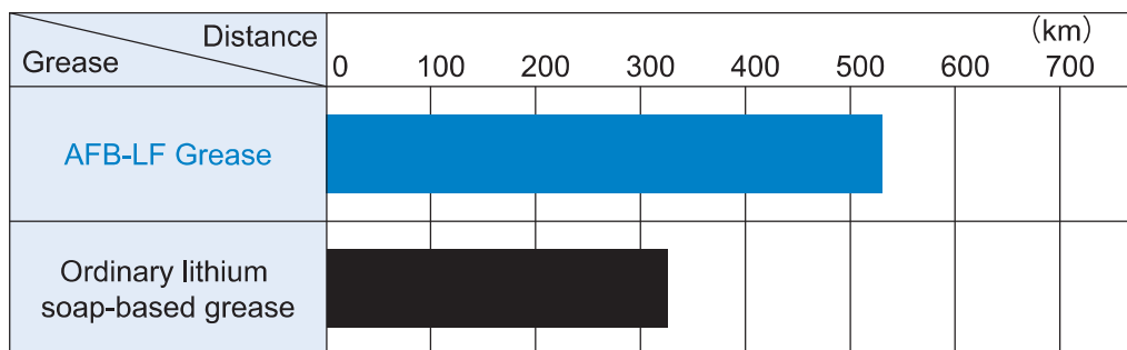
Travel distance until flaking occurs
