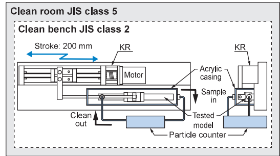
Testing device
