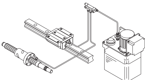
Fig.2 Forced lubrication method
